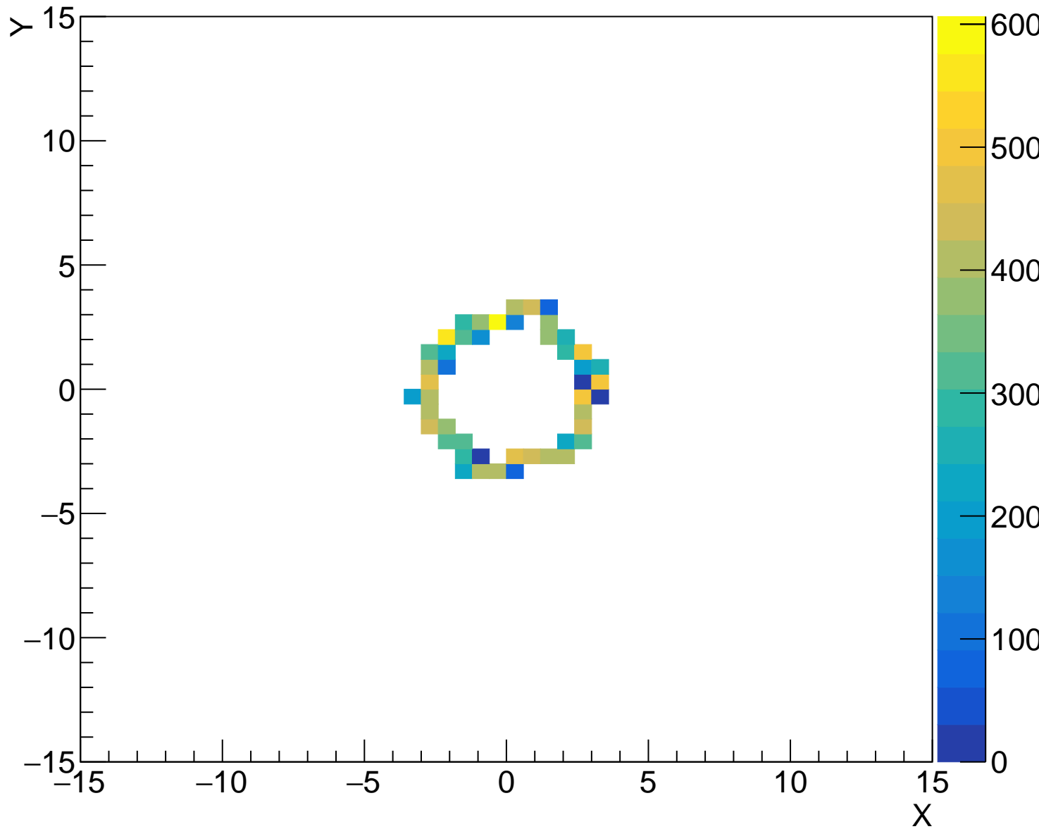
dedx XY map (PXBL1)
