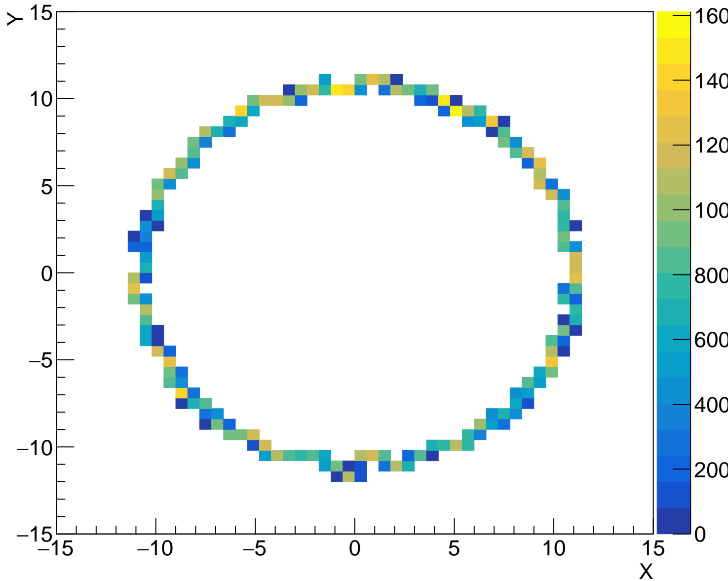
dedx XY map (PXBL3)
