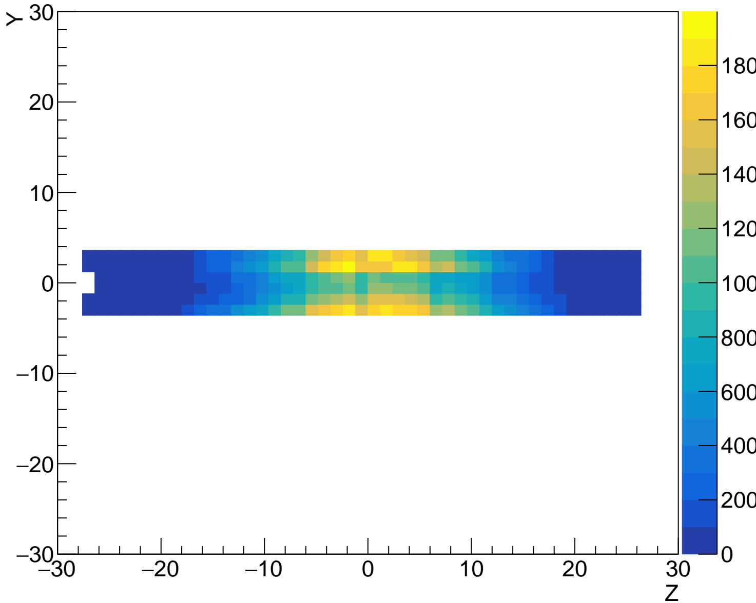
dedx YZ map (PXBL1)
