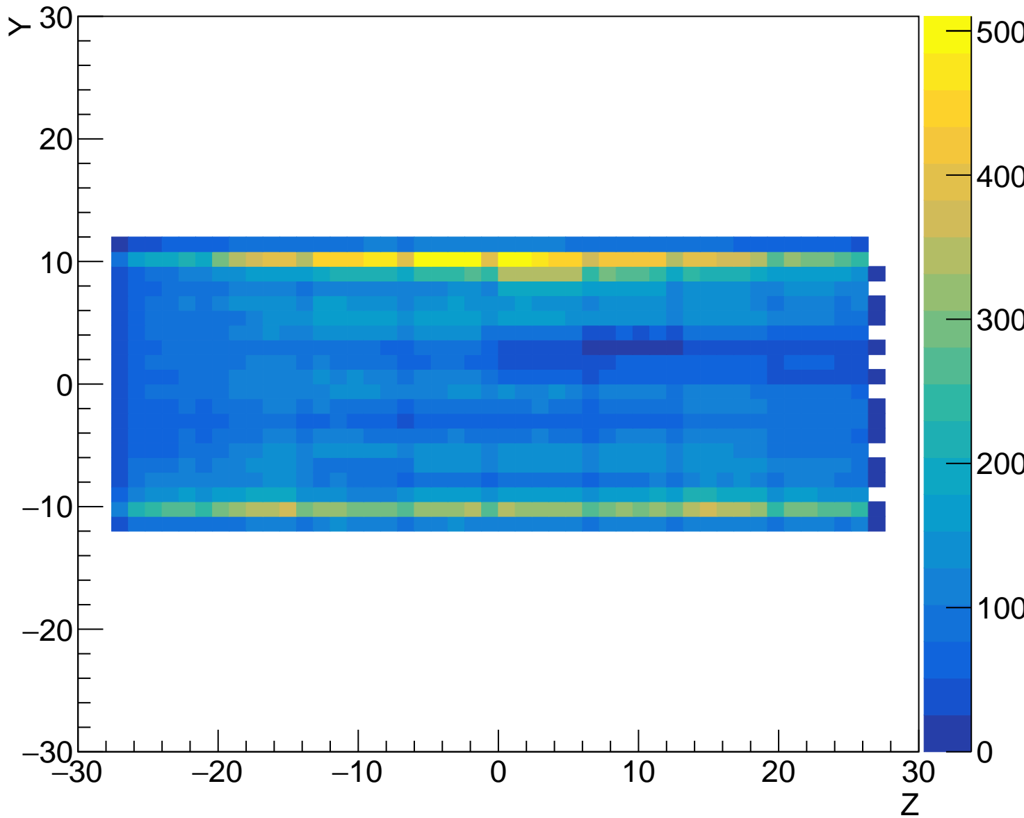
dedx YZ map (PXBL3)
